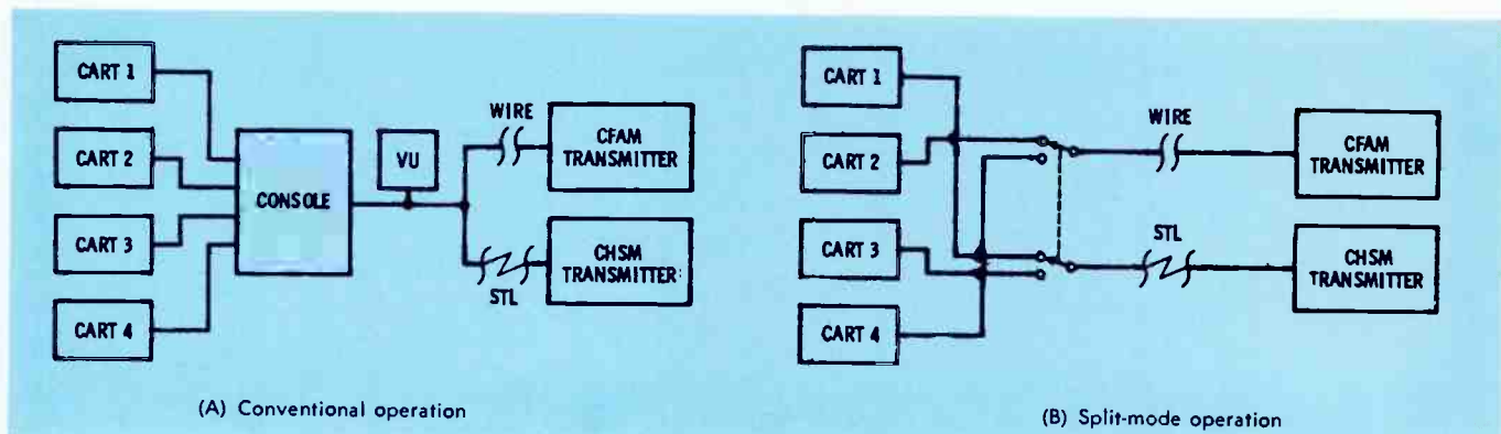
Fig. 2. Commercial spots for the system originate in four cartridge units and can be delivered to either operation.
