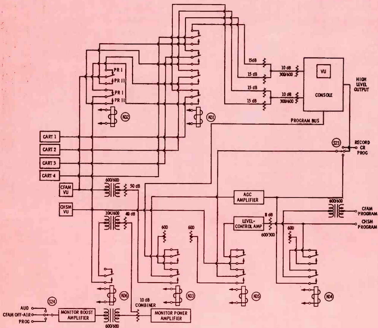
Fig. 3. Audio circuit includes cartridge units, console, level-control amplifier, AGC amplifier, relays, and connections.
